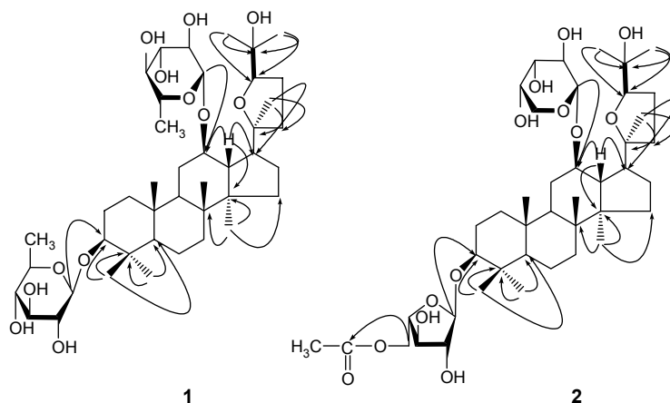
Figure 2. Selected HMBC correlations of compounds 1 and 2 .
